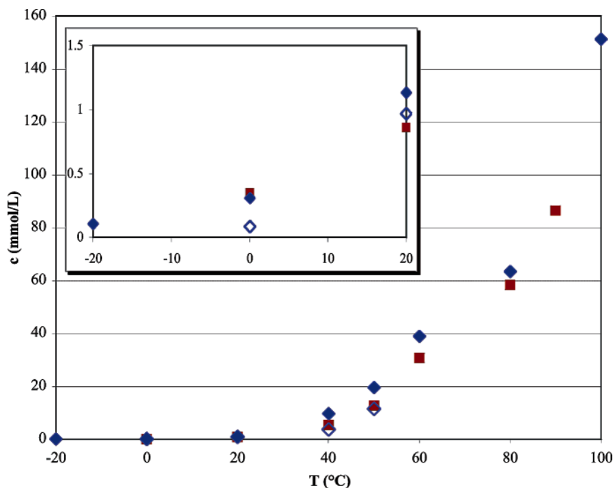
Figure 2. Solubilities of fluoruous phosphines in n -octane as a function of temperature. \blacklozenge 1a , GC assay; \diamond 1a , 31 P NMR assay; \blacksquare 1b , GC assay.
