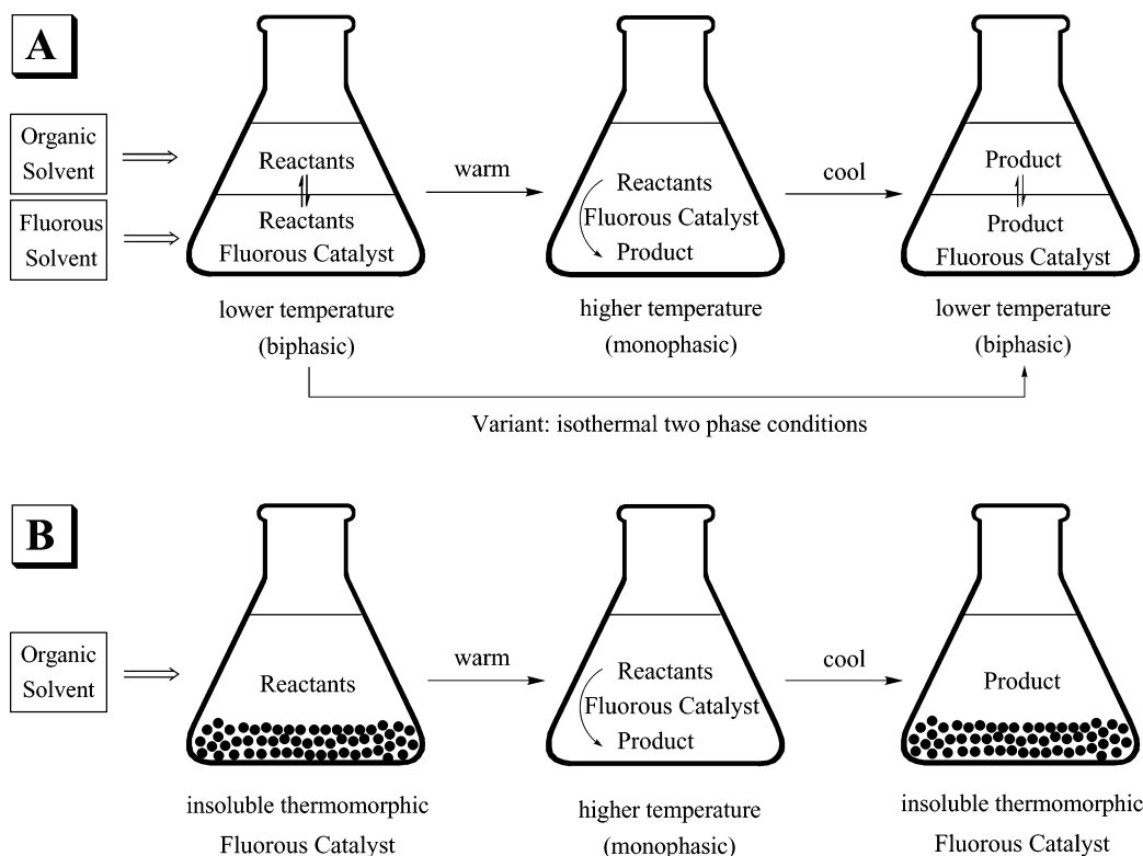
Figure 1. Possible protocols for fluorous biphasic catalysis: (A) recycling by liquid/liquid phase separation; (B) recycling by liquid/solid phase separation.
