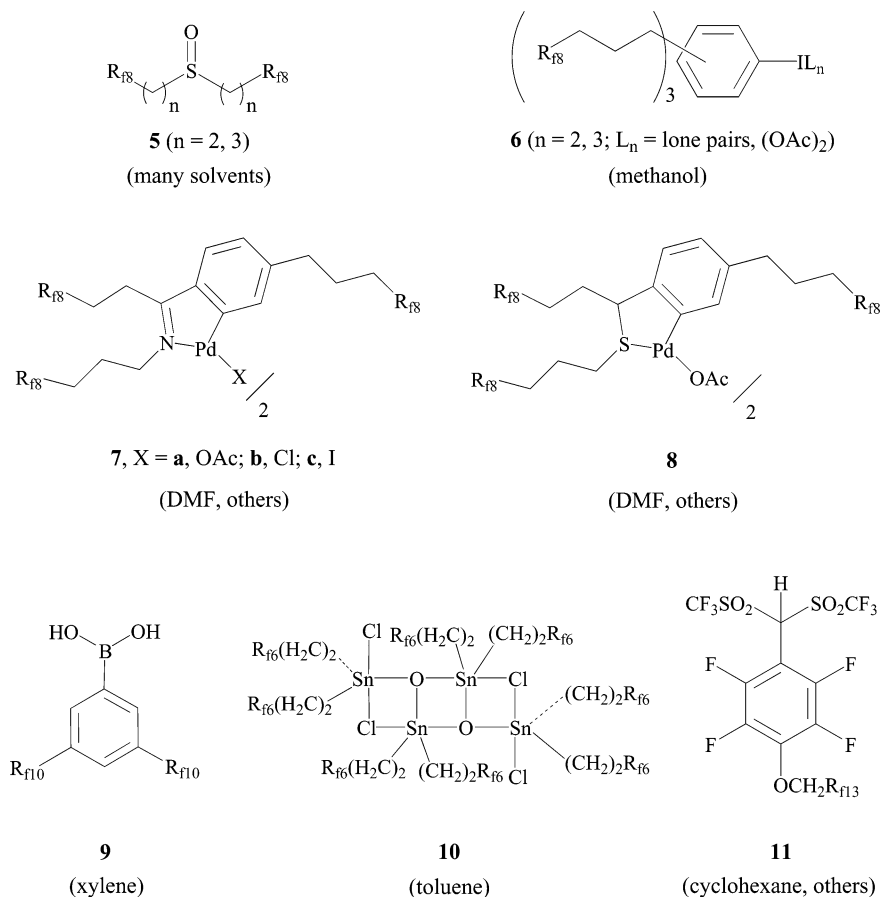
Figure 7. Some fluorous compounds with very low solubilities at room temperature, but much higher solubilities at elevated temperatures.
